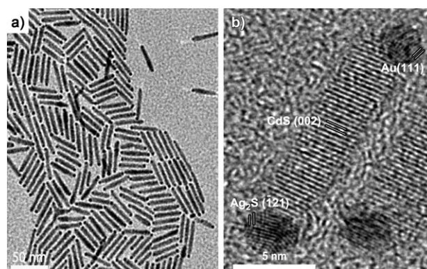
Figure 5. a) TEM image of seeded \text{CdSe/CdS} nanorods with Au nanoparticles at one end and \text{Ag}_2\text{S} nanoparticles at the other end. b) HRTEM image showing the visible lattice fringes of the \text{Ag}_2\text{S} {121} and Au {111} planes with measured d spacings of 0.26 nm and 0.24 nm, respectively.
